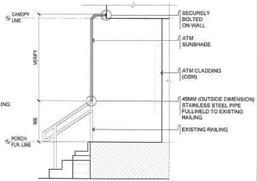
2 ELEVATION DETAIL A-1 SCALE 1:40 METERS
