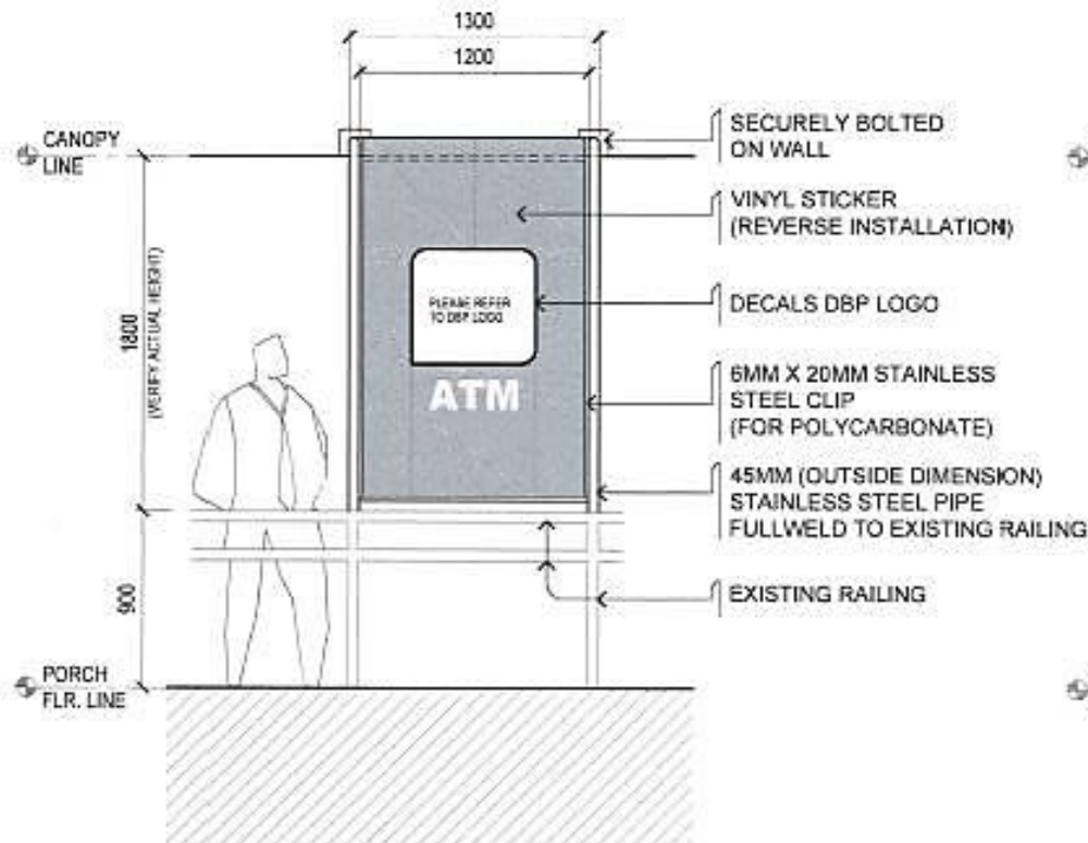
1 SECTION DETAIL A-1 SCALE 1:40 METERS
