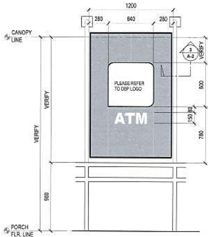
1 A-2 SCALE 1:30 METERS
