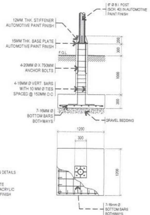
FOOTING DETAILS
