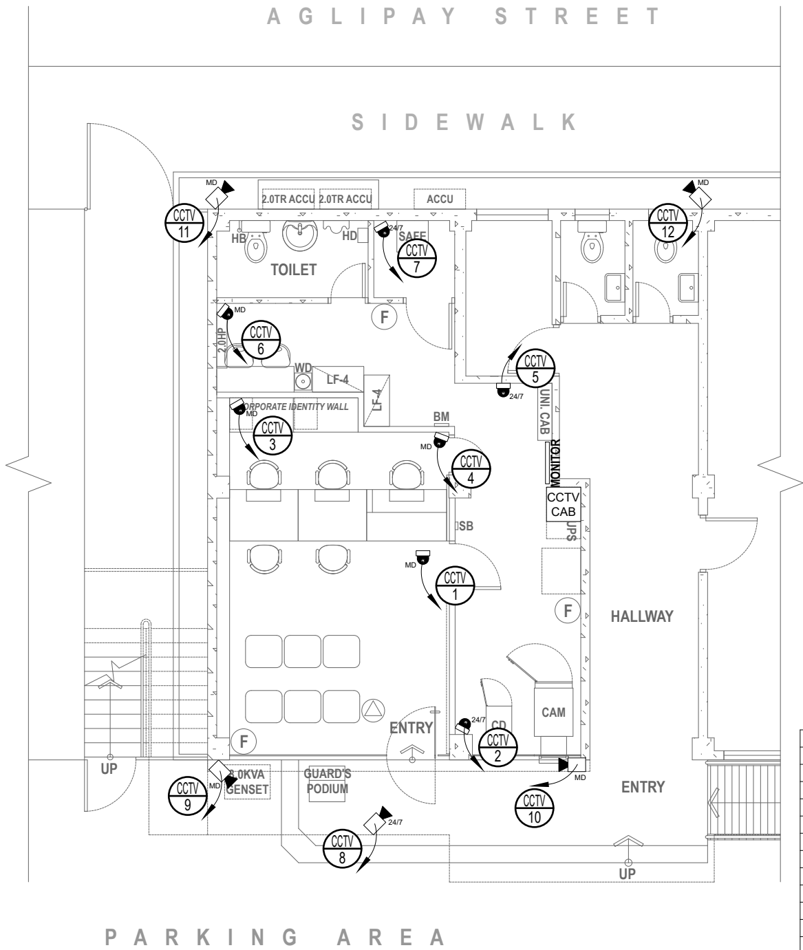
1 ECE-1 SCALE 1:50 METERS CCTV SURVEILLANCE SYSTEM LAYOUT
