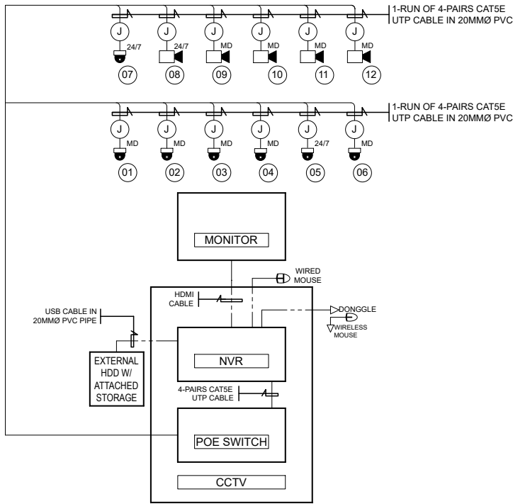
2 ECE-1 SCALE 1:50 METERS CCTV SURVEILLANCE SYSTEM LINE DIAGRAM
