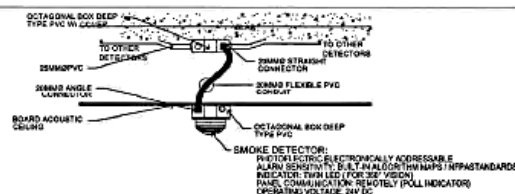
4 MOUNTING DETAILS ECE-1 NOT TO SCALE
