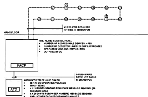
2 RISER DIAGRAM ECE-1 NOT TO SCALE
