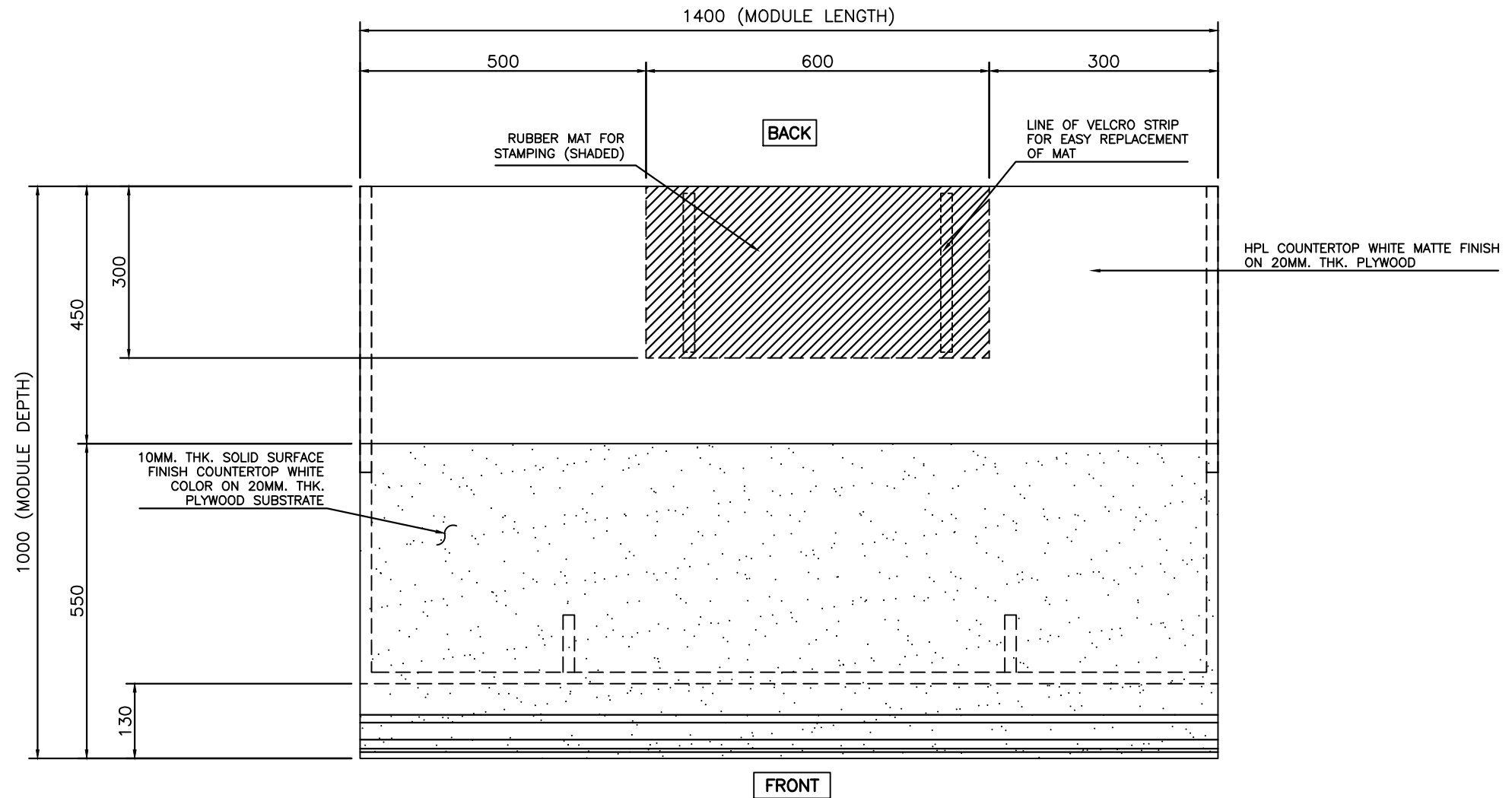
UPPER COUNTERTOP PLAN
