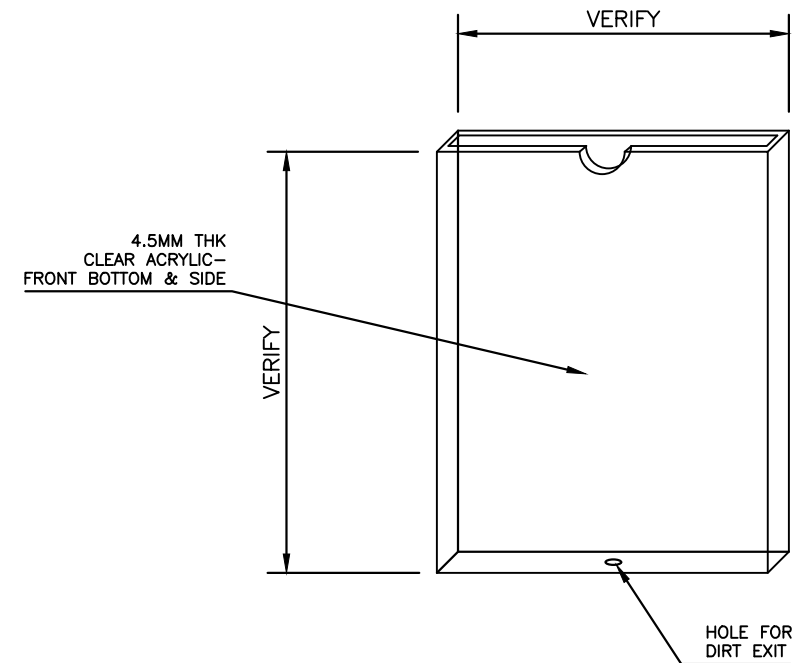
ISOMETRIC OF ACRYLIC INSERTS
