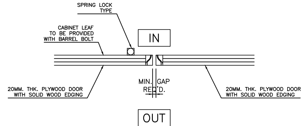
CABINET DOOR DETAIL
