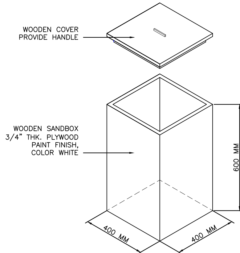
ISOMETRIC
