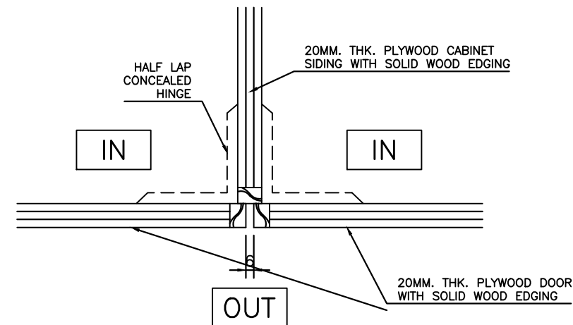
MID CABINET TO CABINET DOOR CONNECTION
