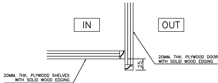
FINGER FULL DETAIL
