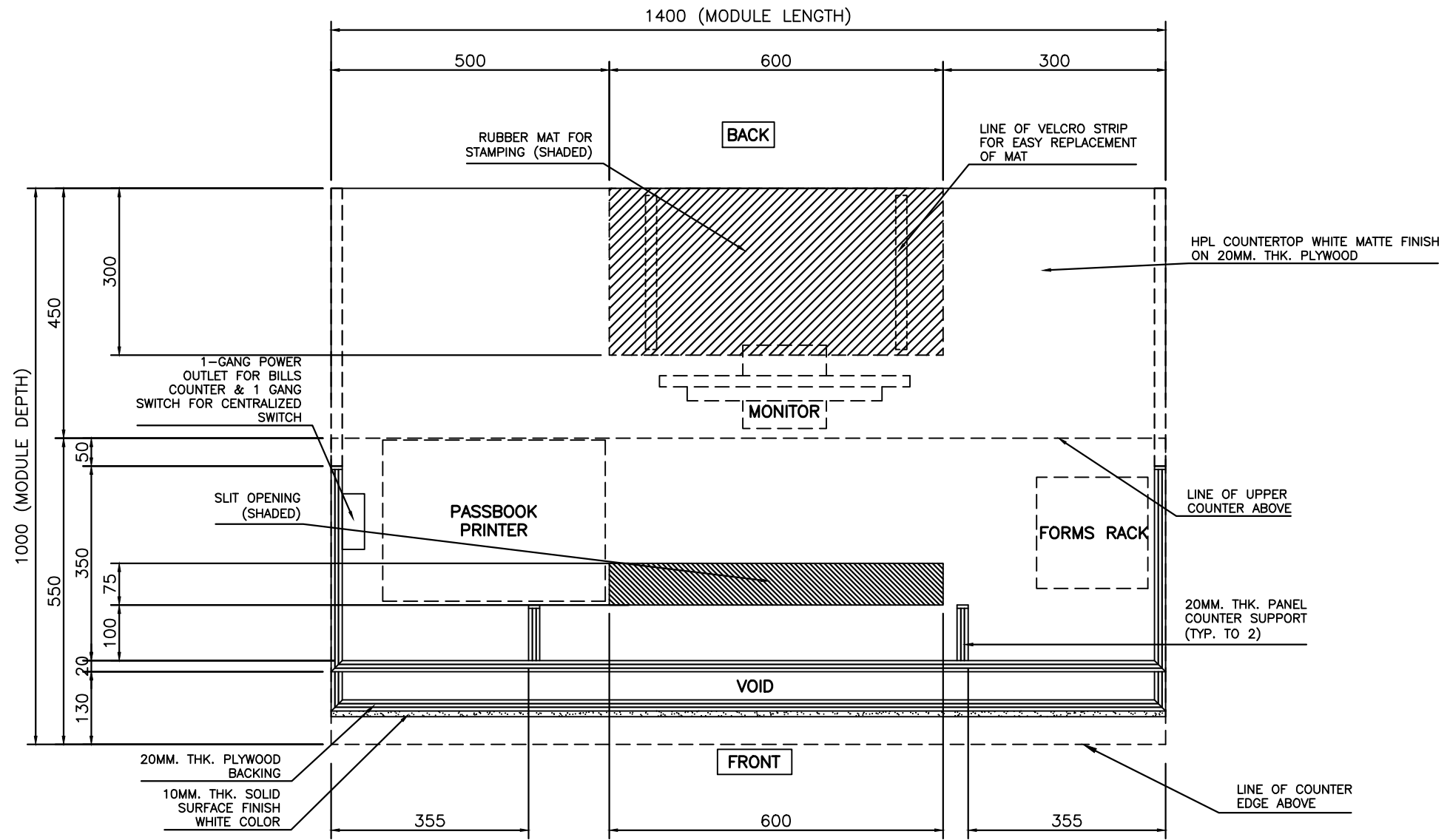
LOWER COUNTERTOP PLAN
