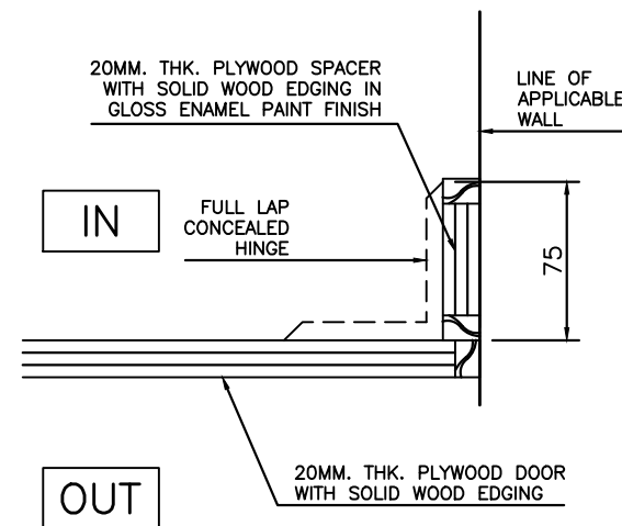
WALL EDGE TO CABINET DOOR CONNECTION
