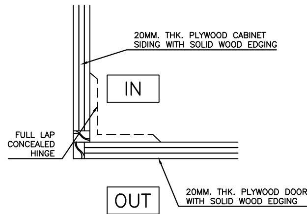
CABINET EDGE TO CABINET DOOR CONNECTION
