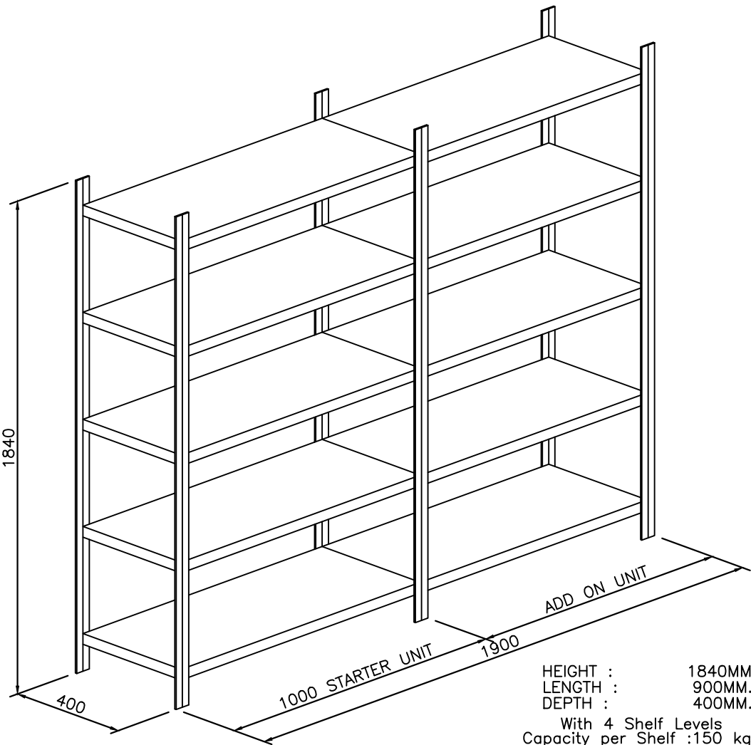
STEEL SHELVES
