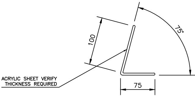
SIDE ELEVATION
