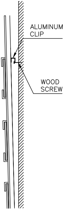
SECTION
