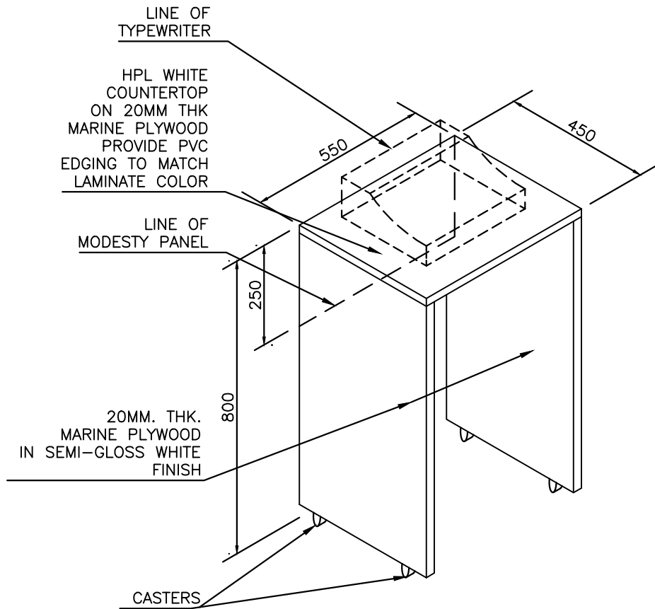
TYPING TABLE ISOMETRIC
