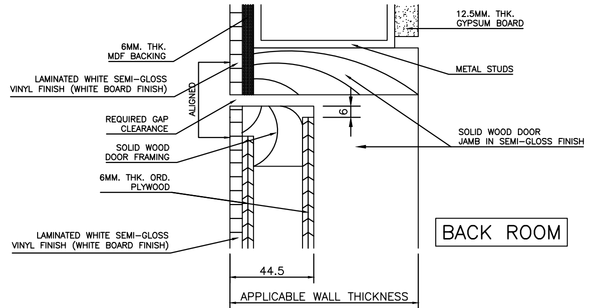
"D" - DETAIL
