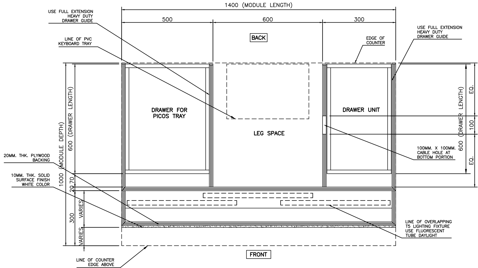
BOTTOM PLAN
