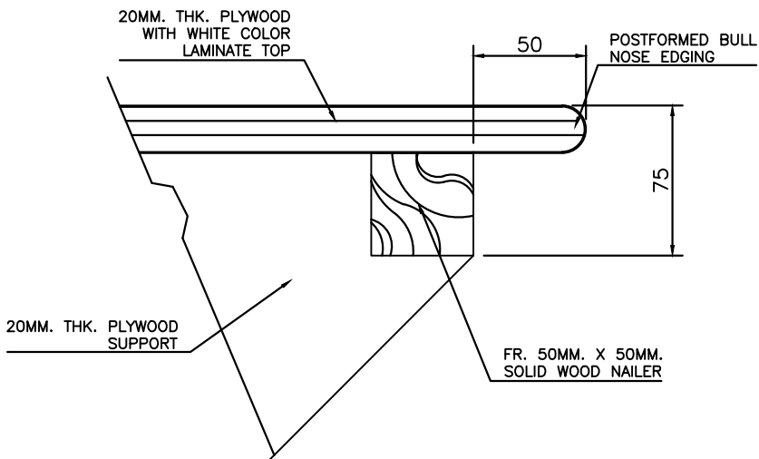
"A" DETAIL
