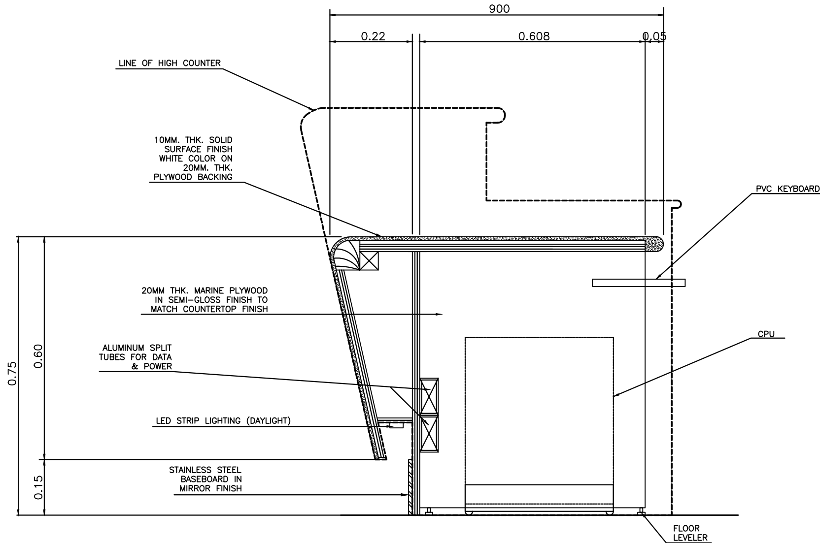
SECTION ALONG CPU
