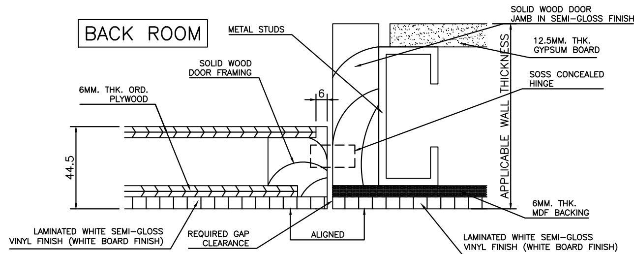
"C" - DETAIL
