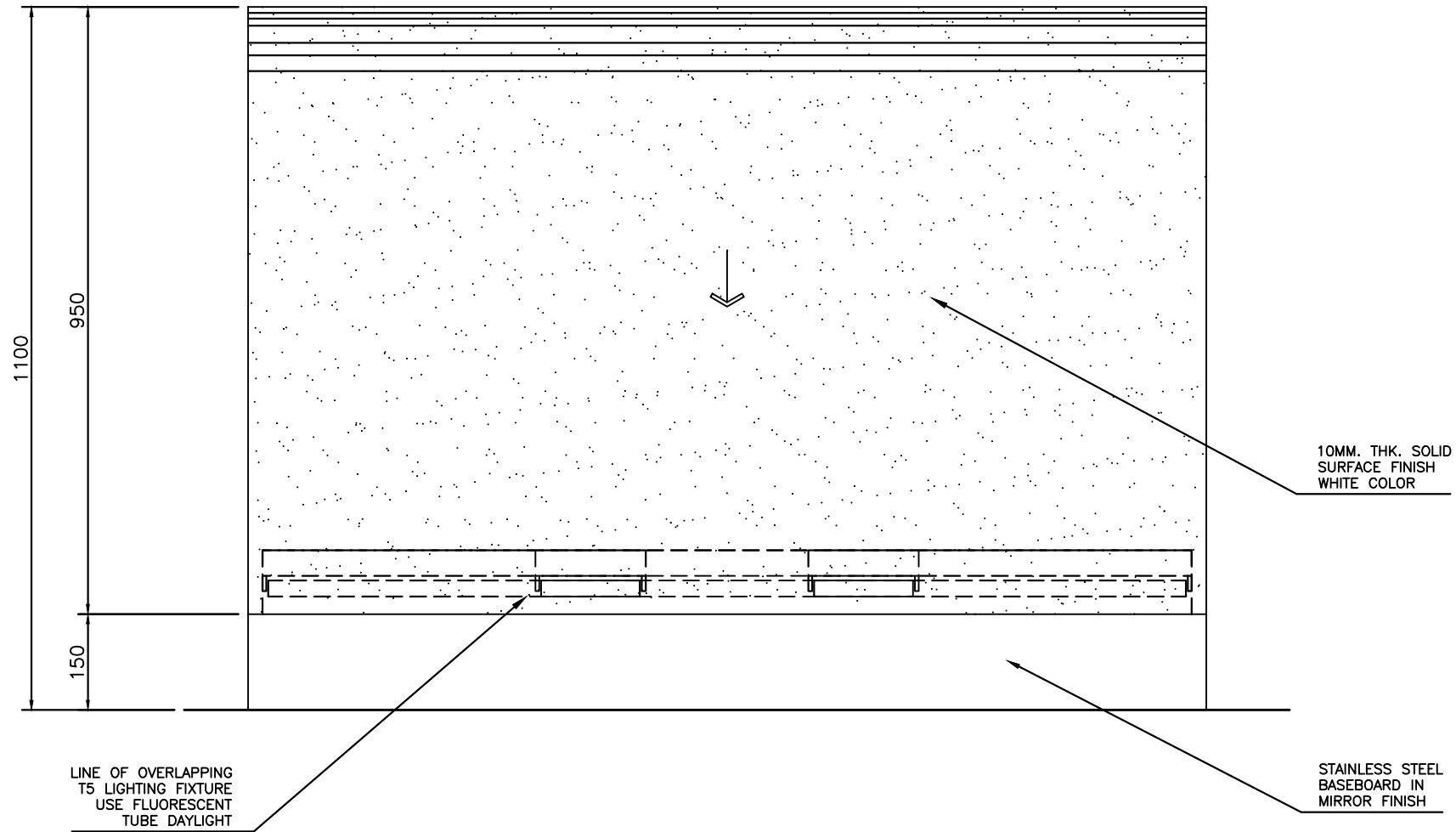
FRONT ELEVATION
