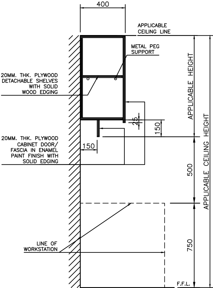
BACKROOM OVERHEAD CABINET DETAILED SECTION
