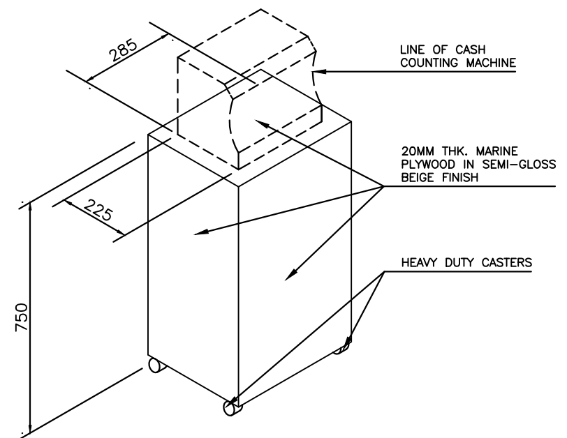
MONEY COUNTER MODULE
