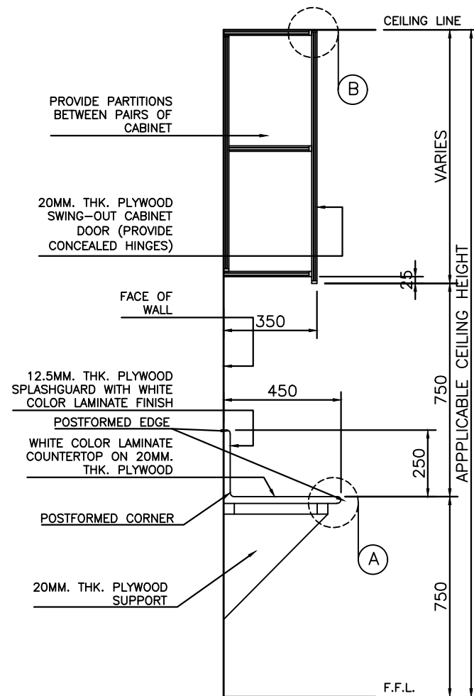
PANTRY COUNTER WITH OVERHEAD CABINET SECTION
