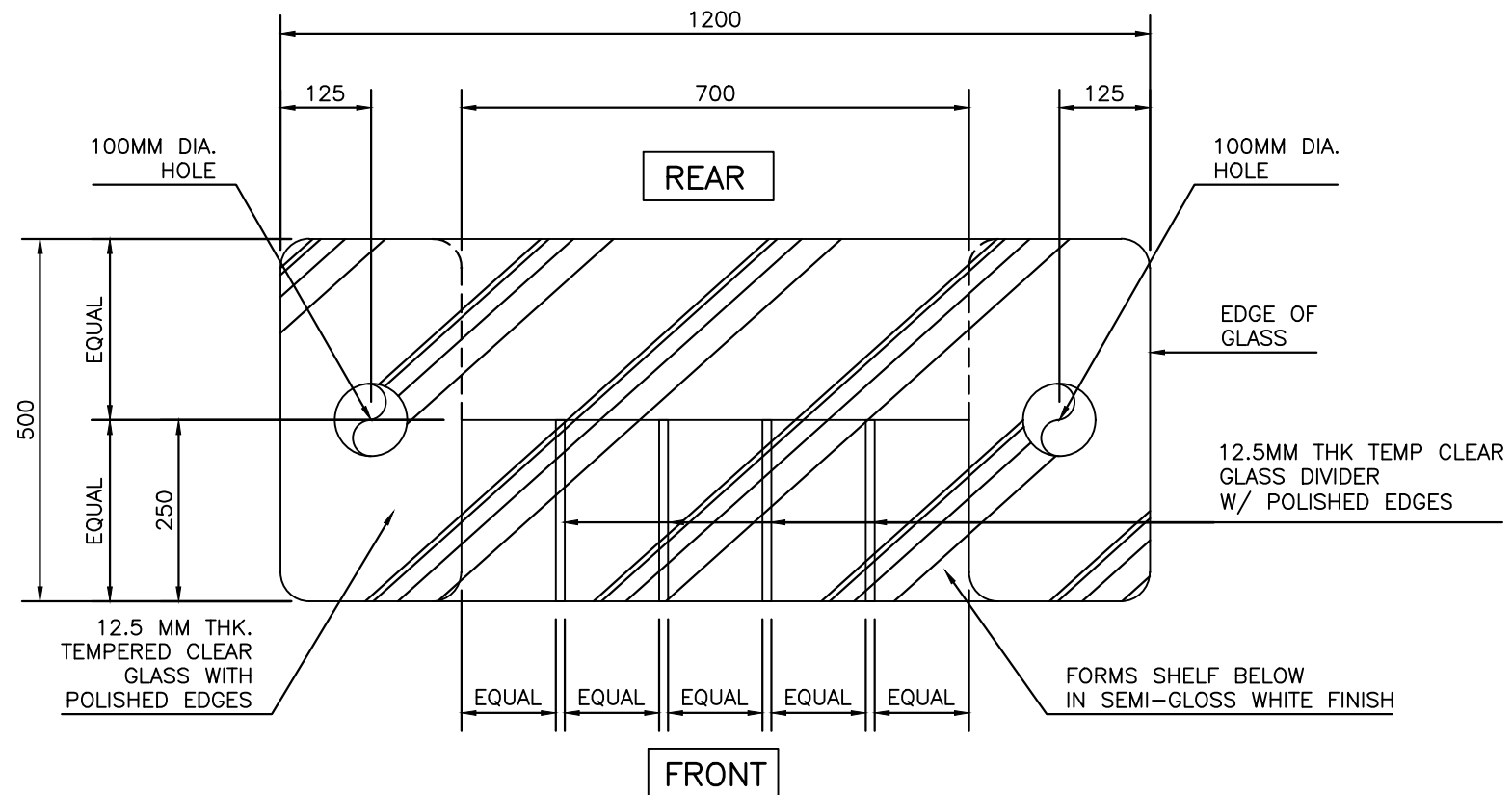
COUNTER TOP PLAN
