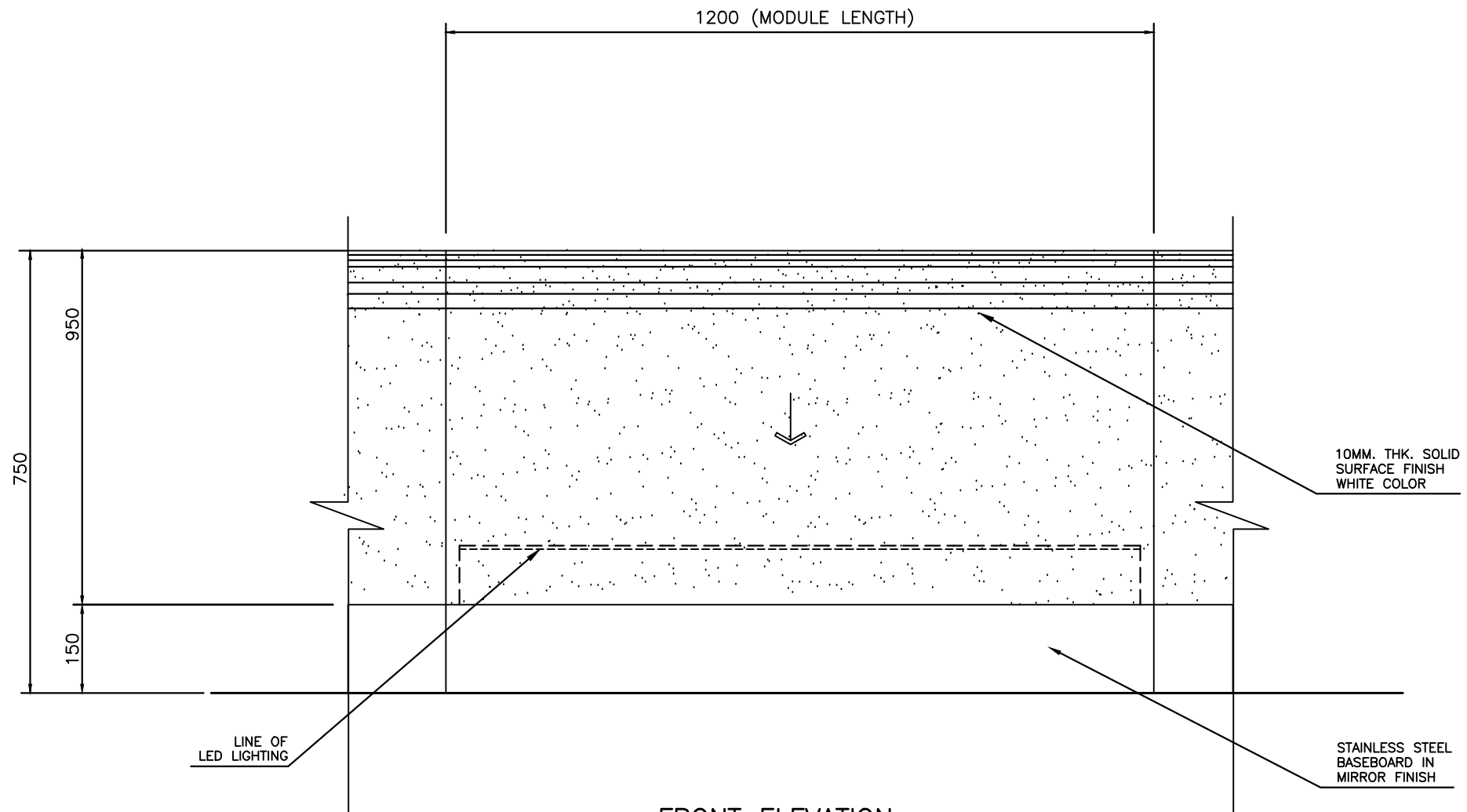
FRONT ELEVATION
