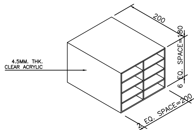
ISOMETRIC-FORMS RACK
