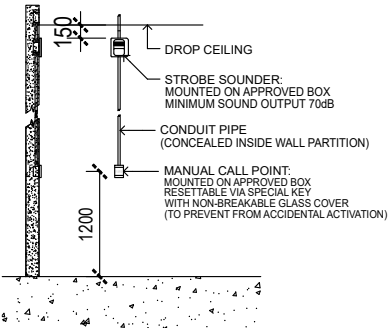
3 ECE-1 NOT TO SCALE MOUNTING DETAILS ADDRESSABLE MANUAL CALL POINT WITH STROBE SOUNDER
