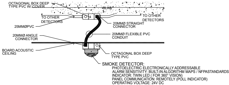
4 ECE-1 NOT TO SCALE MOUNTING DETAILS ADDRESSABLE SMOKE DETECTOR
