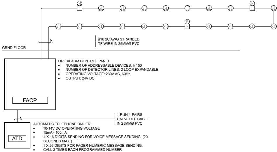
2 ECE-1 NOT TO SCALE RISER DIAGRAM FIRE DETECTION ALARM SYSTEM
