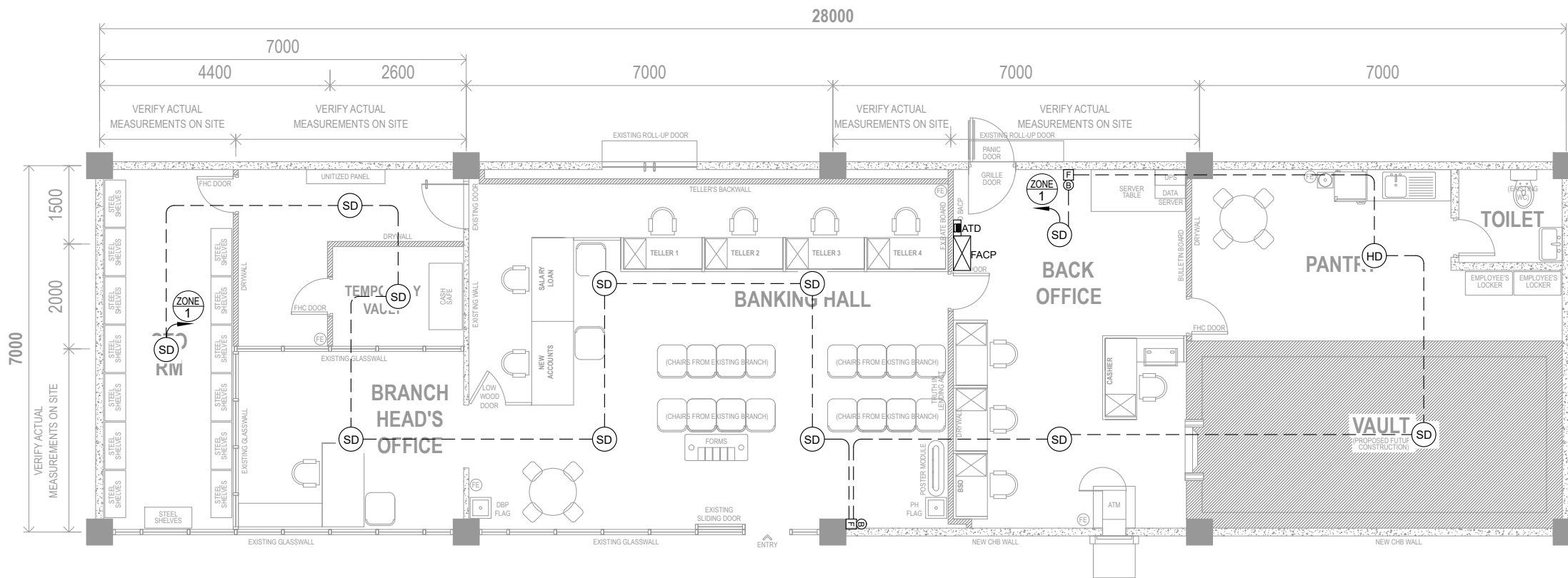
1 FIRE DETECTION ALARM SYSTEM LAYOUT ECE-1 SCALE 1:100 MTS
