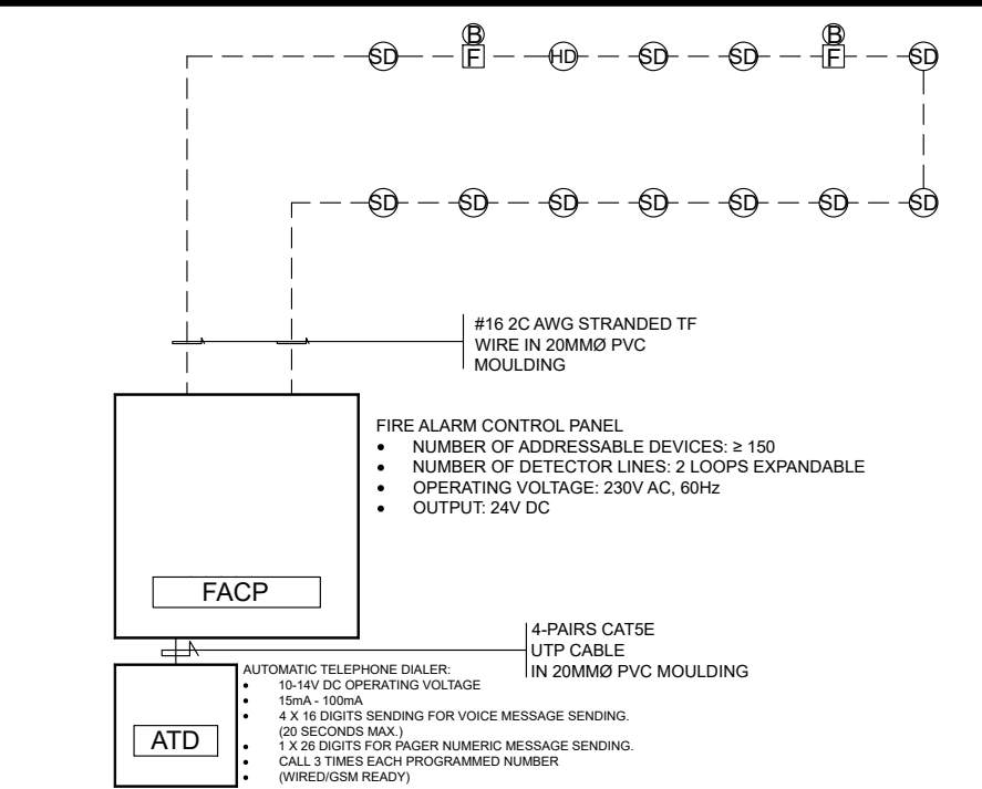
2 FIRE DETECTION ALARM SYSTEM RISER DIAGRAM ECE-1 SCALE NTS
