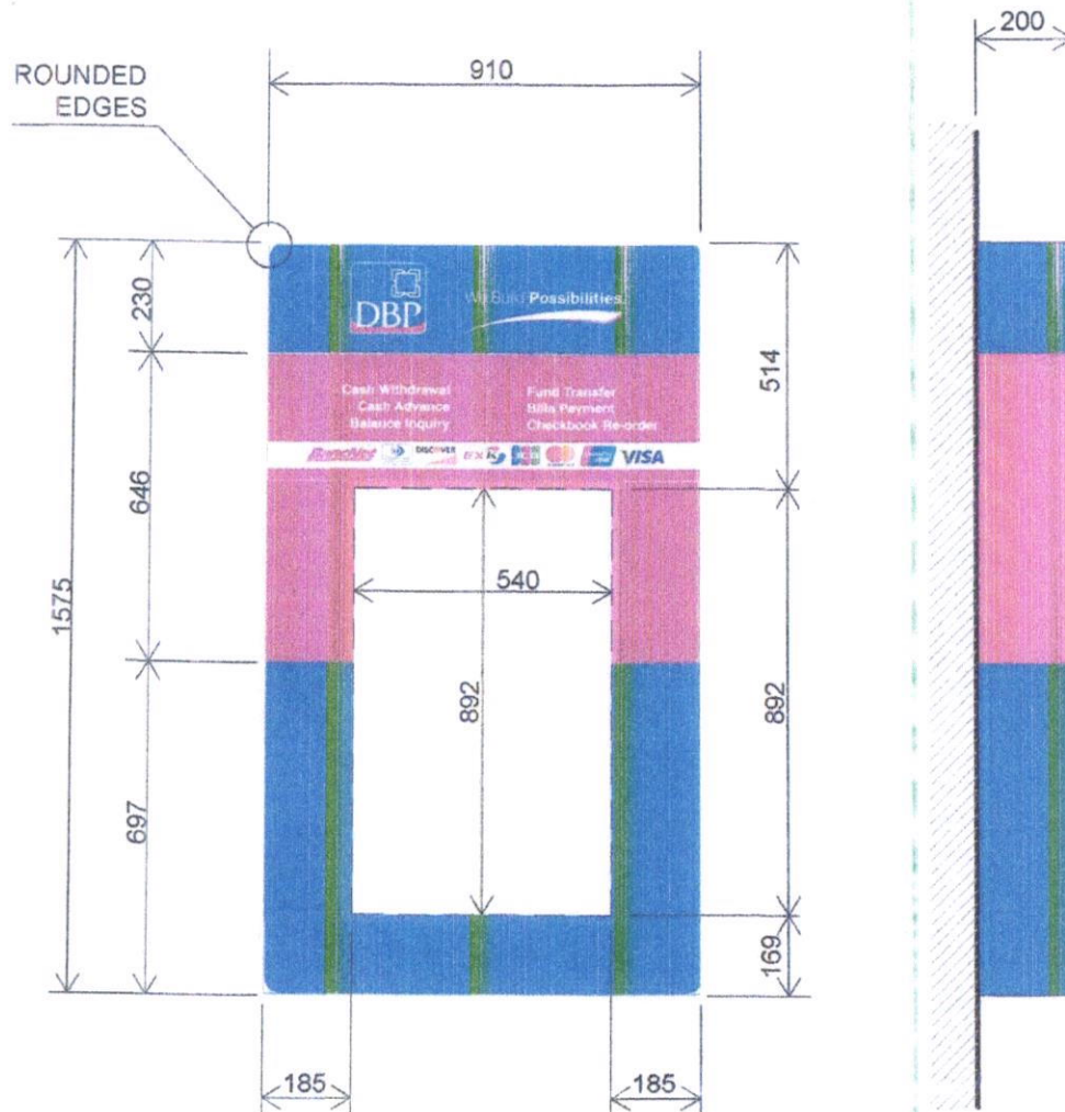
FRONT ELEVATION/SECTION
