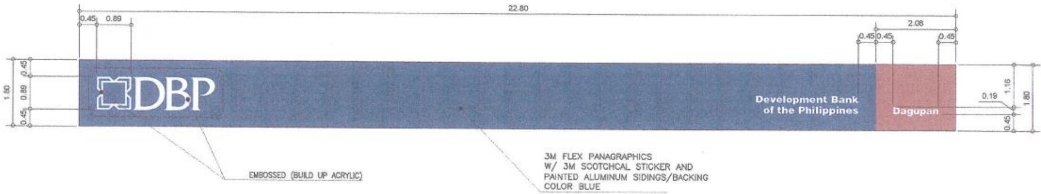
FACADE HORIZONTAL SIGNAGE ELEVATION
