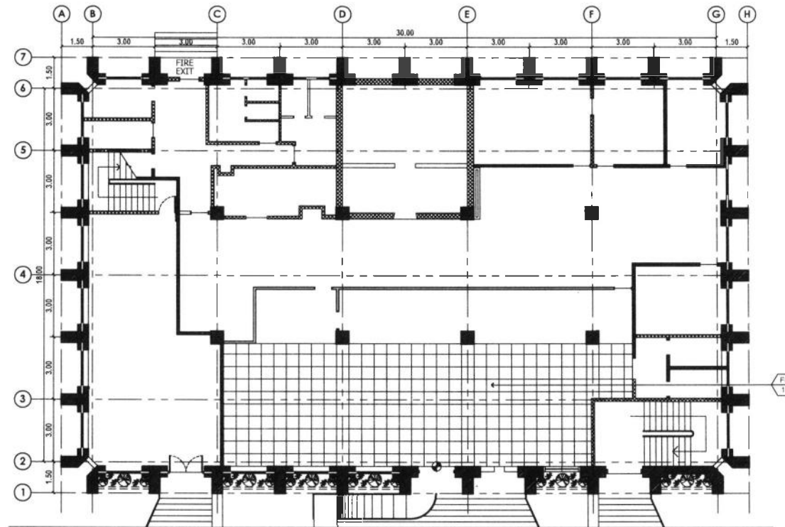
1 FLOOR PATTERN LAYOUT A-1 SCALE 1:100 METERS
